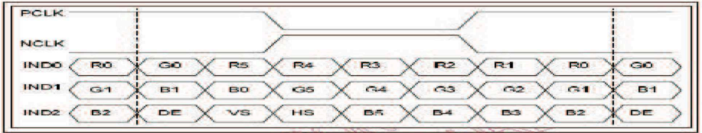
6-bit LVDS Input Timing chart
