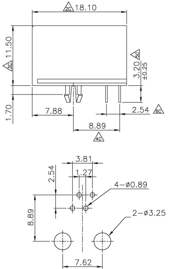
PCB LAYOUT/TOP VIEW
