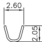
B-B SEC
