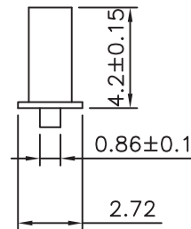
C-C SEC
